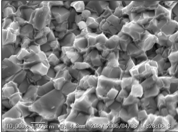
RD series microstructure via Scanning Electron Microscope
